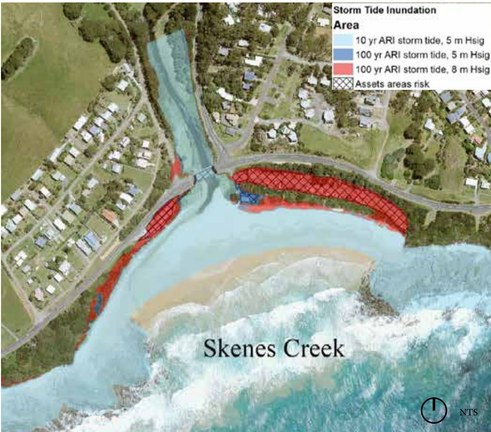
Figure 8. Skenes Creek Inundation and Risk to Assets. Source: Apollo Bay, Skenes Creek & Marengo CIP - Issues and Opportunities Paper: Coastal study prepared by WaterTechnology.
