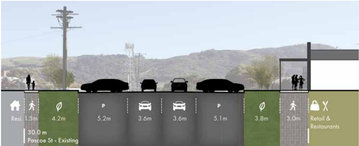
Figure 23. Pascoe Street A-A' (Between Moore St And Nelson St) - Existing Cross Section PLEASE NOTE: Dimensions indicative only and based off Nearmap Aerial.
