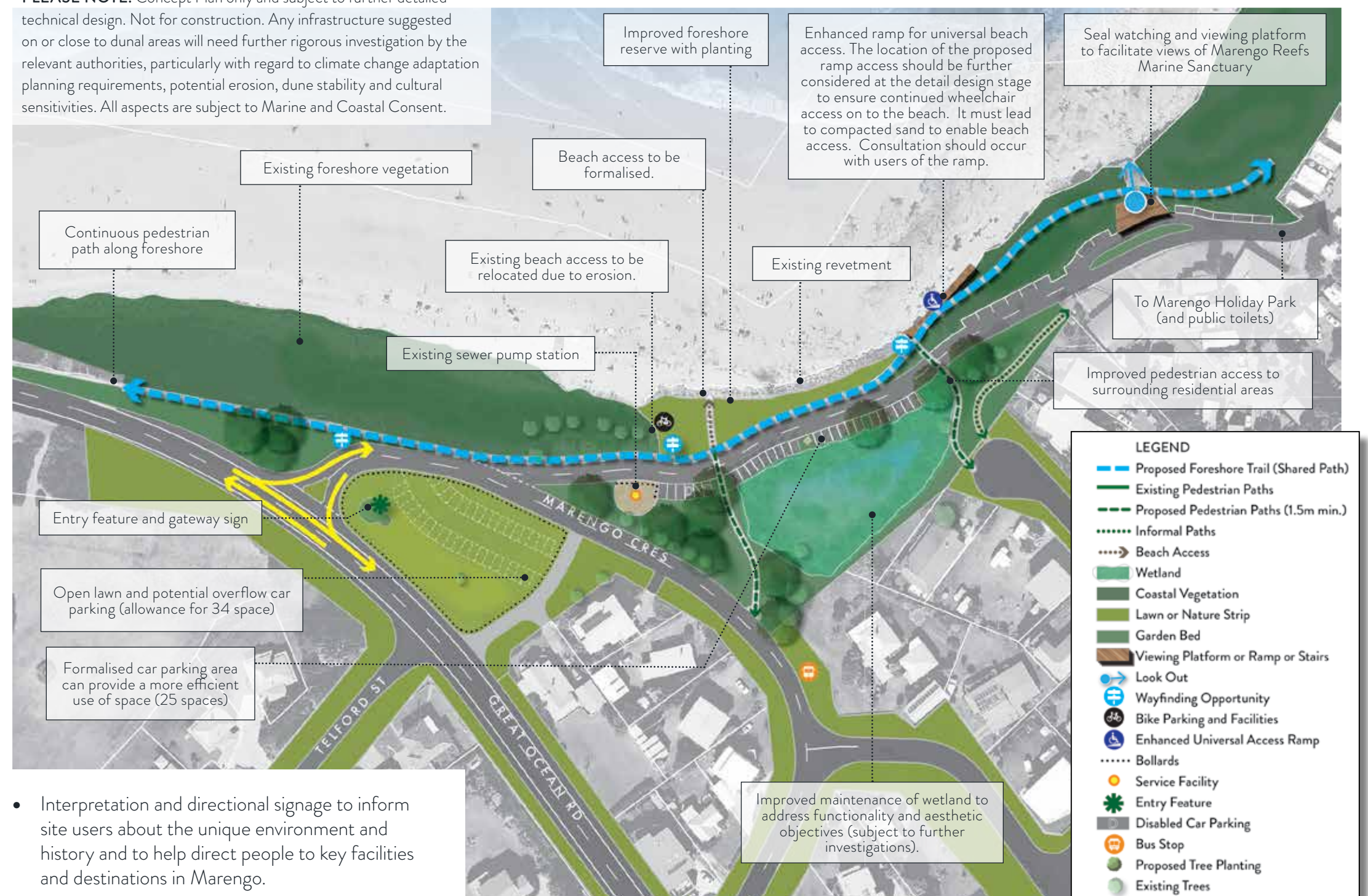
Figure 14. Marengo Foreshore Master Plan
