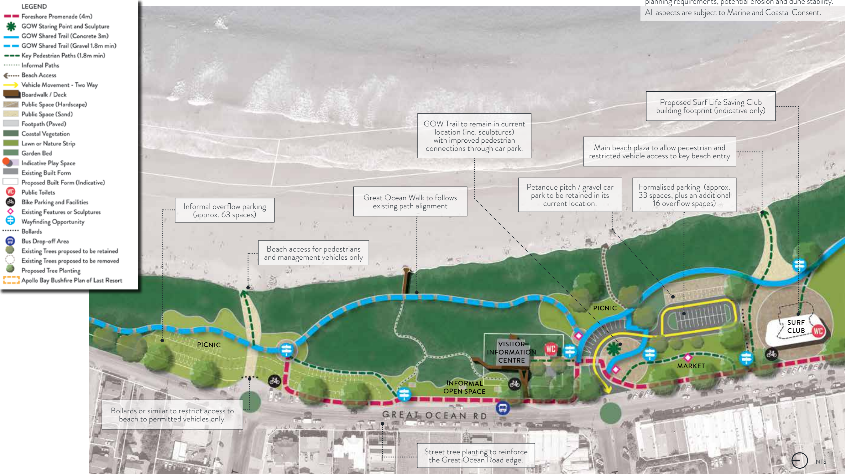
Figure 11. Thomson Street to Surf Club Plan
